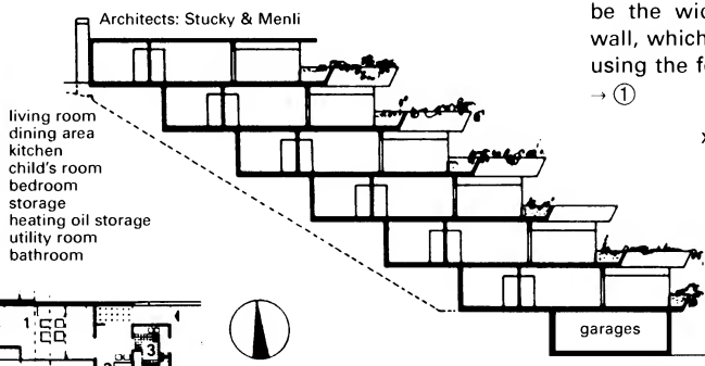
⑨ Section
